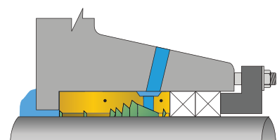
Split Packing Version SpiralTrac (Version P)
