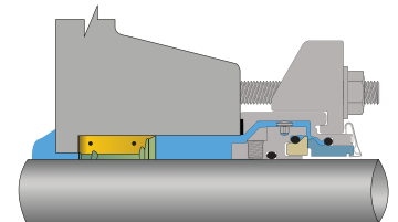
SpiralTrac Version F Type S
