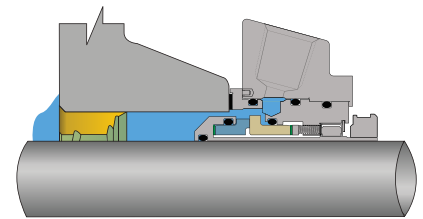
SpiralTrac Version N/D/C Type I
