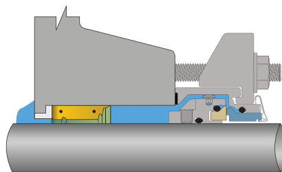
SpiralTrac Version F Type S
