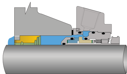
SpiralTrac Version N/D Type A
