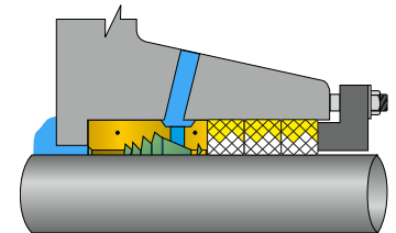
Split Packing Version SpiralTrac (Version P)
