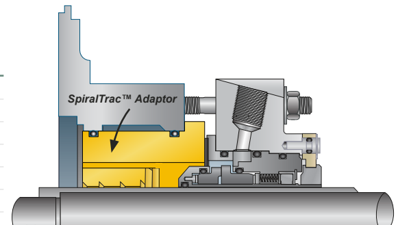
SpiralTrac™ Adaptor with Chesterton S10 Mechanical Seal
