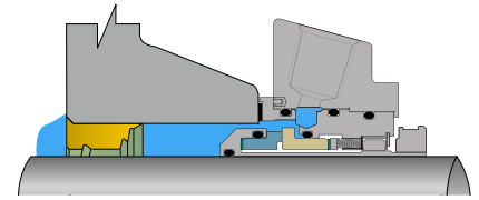
SpiralTrac Version N/D/C Type I
