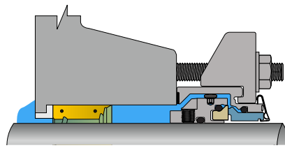
SpiralTrac Version F Type S
