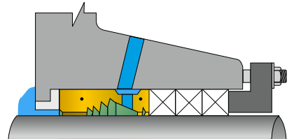
Split Packing Version SpiralTrac (Version P)
