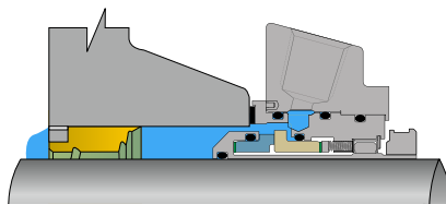
SpiralTrac Version N/D Type A
