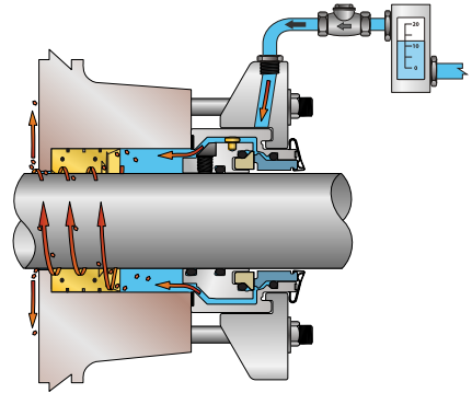
442C Split Seal
