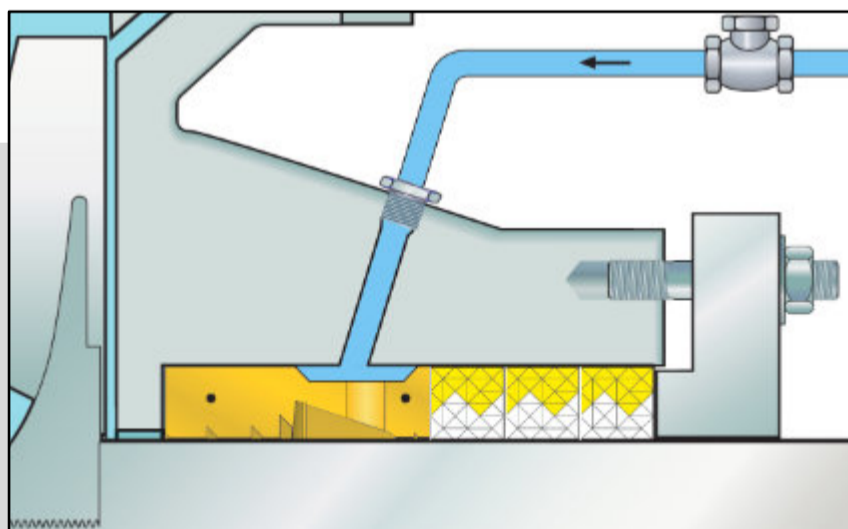
Chesterton SuperSet: SpiralTrac + 3 rings of DualPac 2212
