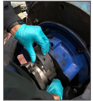
Split Packing Version SpiralTrac being installed
