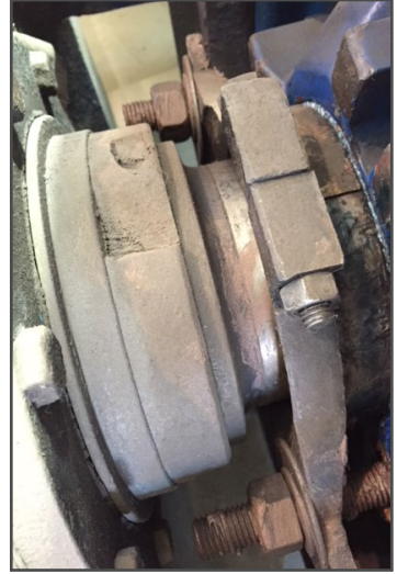
Chesterton SuperSet installed in Larox Filer Pump
